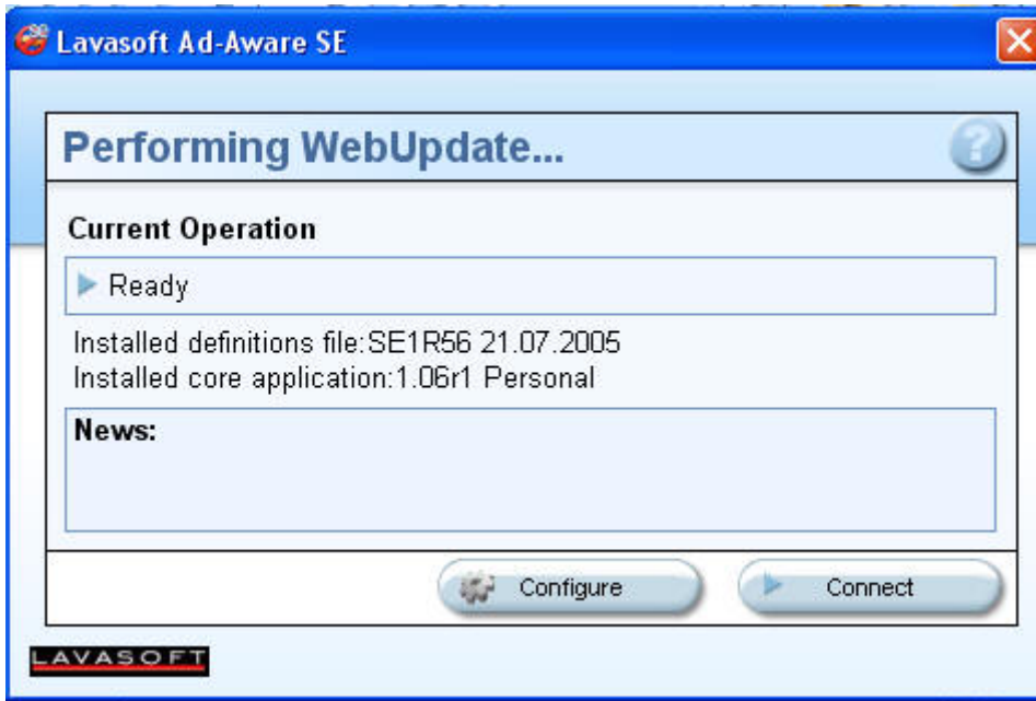
Figure 3. Starting WebUpdate
